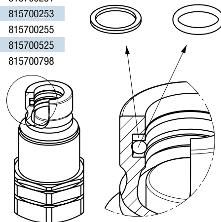
Back-up ring (Teflon®)
